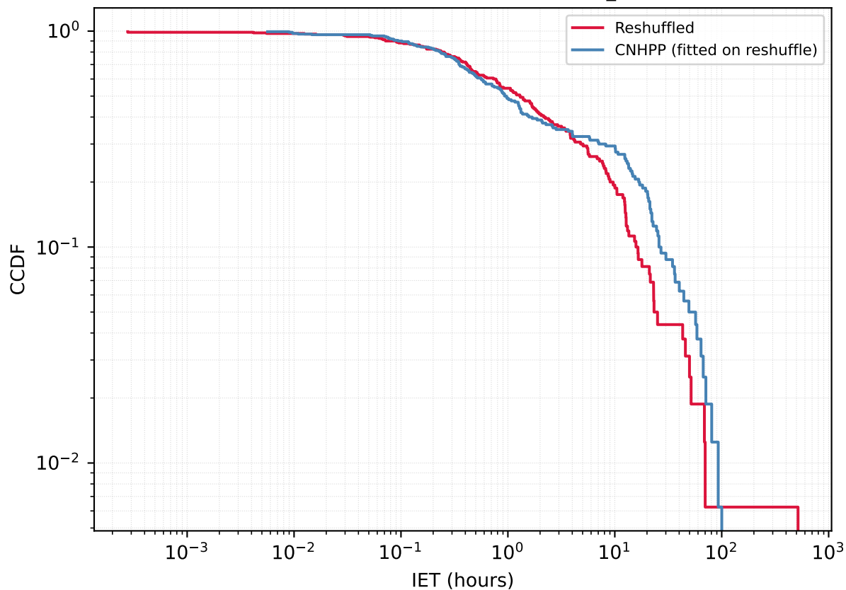
User 791270353 - Reshuffled vs CNHPP A_{\text{fit}}=0.2920
